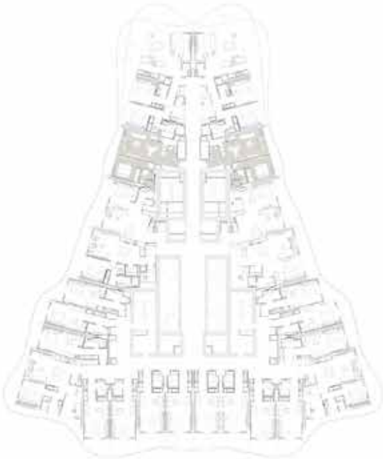
Levels 02-17 Key Plan
